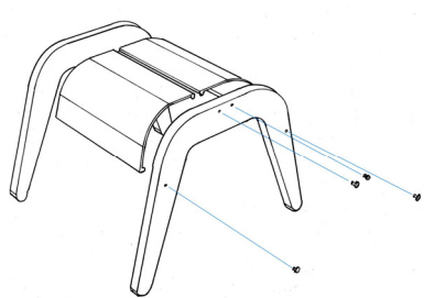
Exploded view
