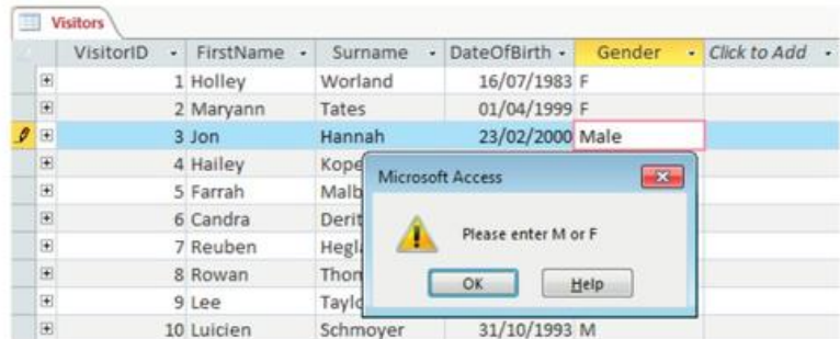
▲ Figure 20.14 A customised validation message helps the user understand what they need to do to enter valid data
