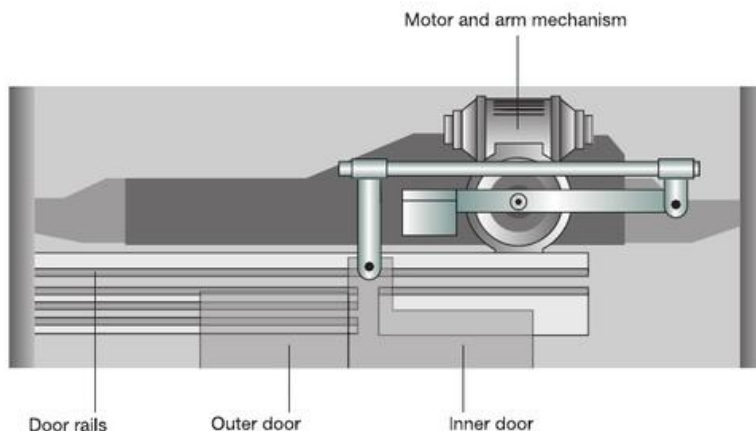
▲ Figure 2.17 Lift doors are opened and closed automatically by control software when a sensor detects that the lift is level with the floor and has stopped
