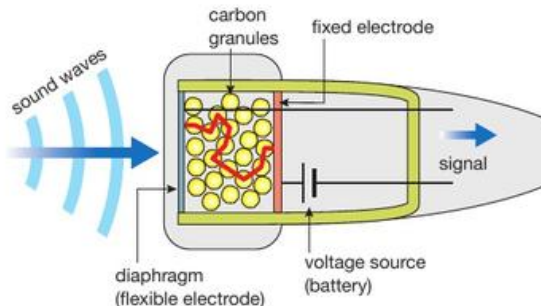
▲ Figure 1.46 Sound waves hitting a microphone and being converted to an electrical signal
